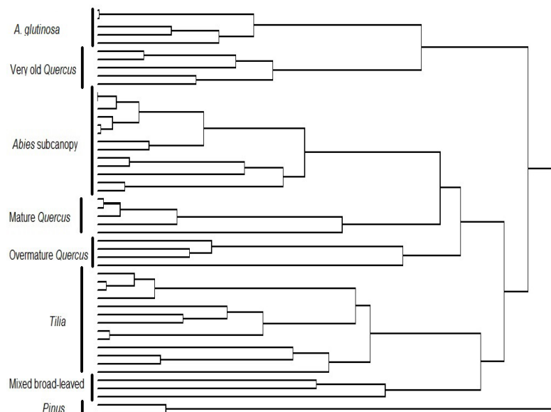
Fig. 2. Cluster analysis of broadleaved forest stands based on tree species composition in age classes.
